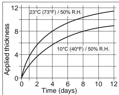
Diagram 1: Curing speed SikaTack® Drive
